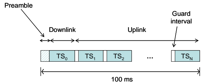
Figure 3. Frame structure.
